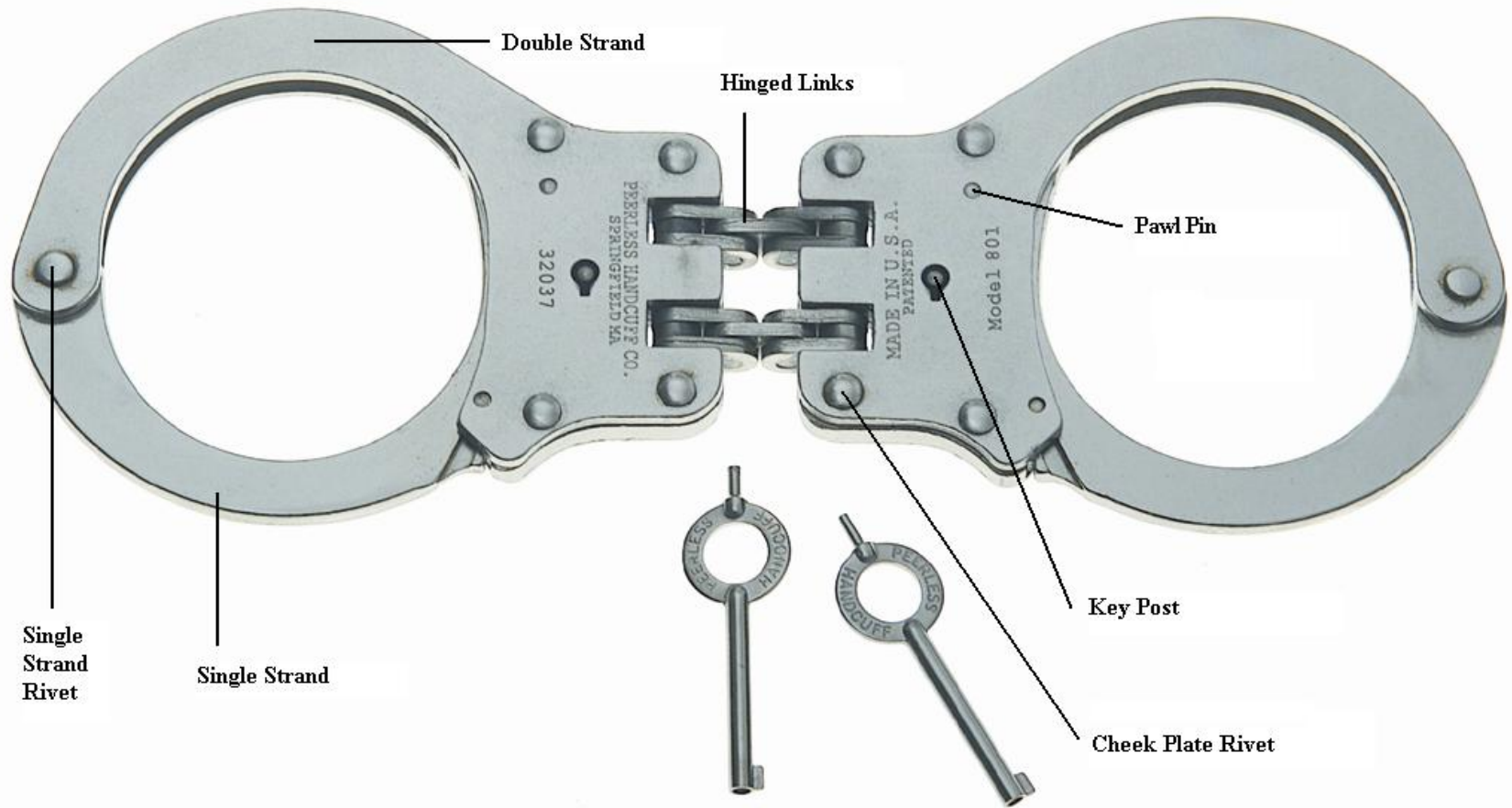
Hinged Handcuff Nomenclature
